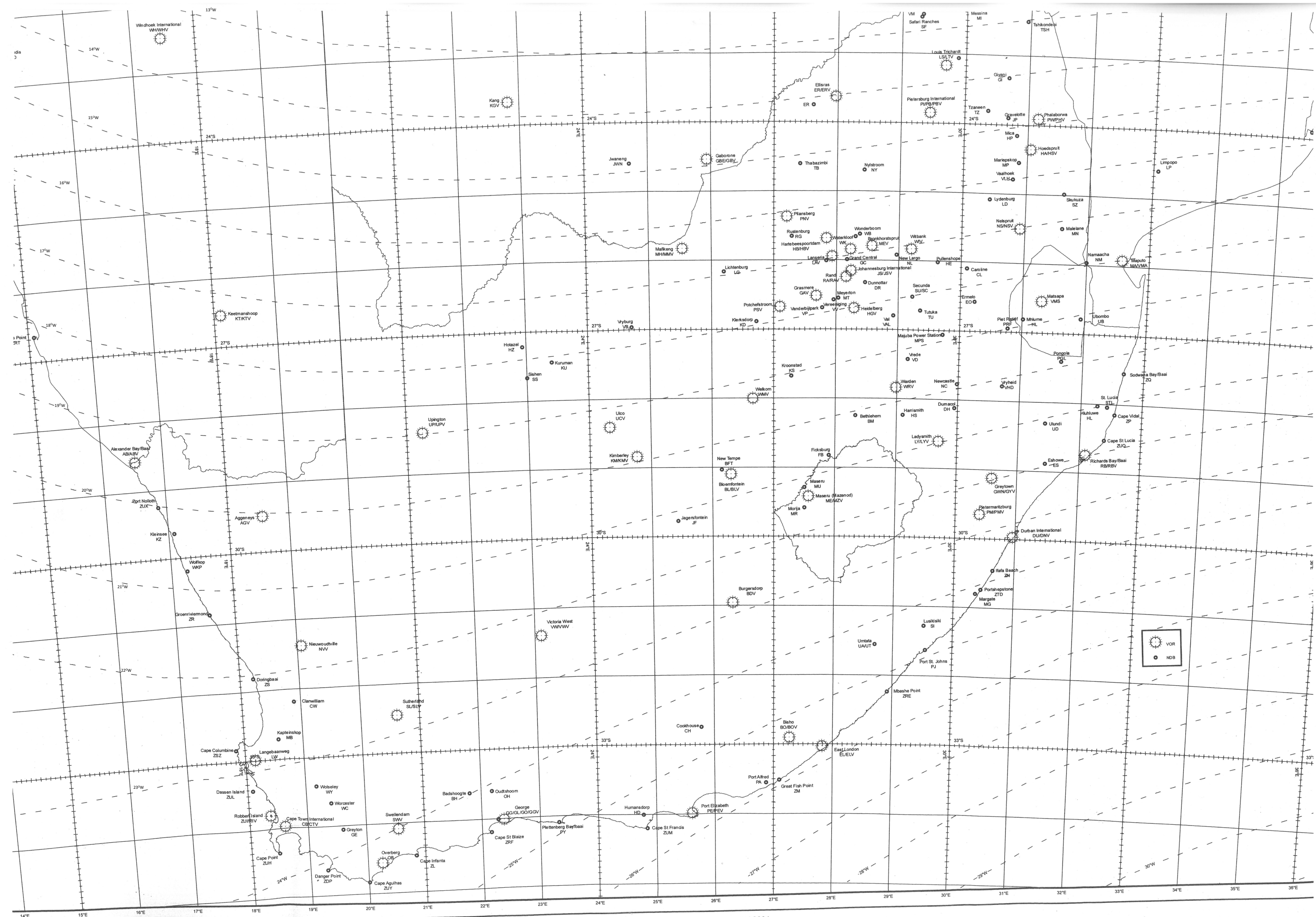
LINES OF EQUAL MAGNETIC VARIATION JULY 2001
